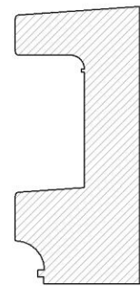
8 BAY WINDOW PROFILE 1 : 10
