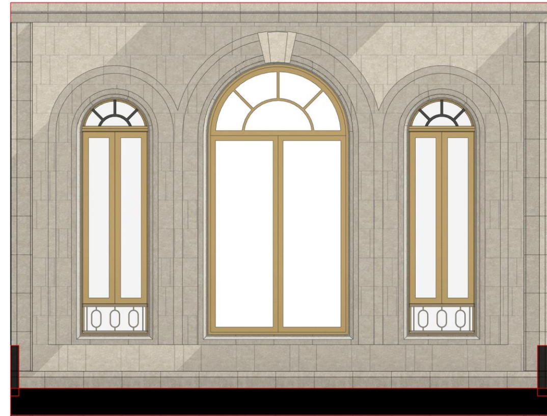
2 MAIN PORTICO WINDOW ELEVATION
