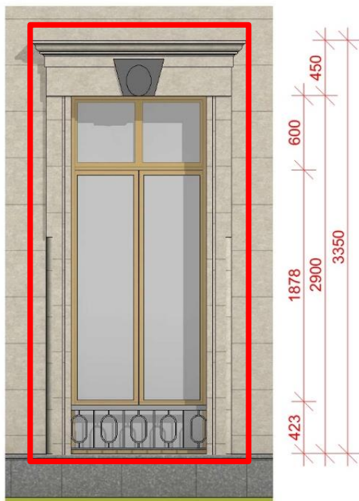
WINDOW ELEVATION A
