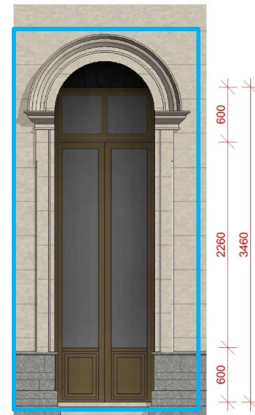
WINDOW ELEVATION D
