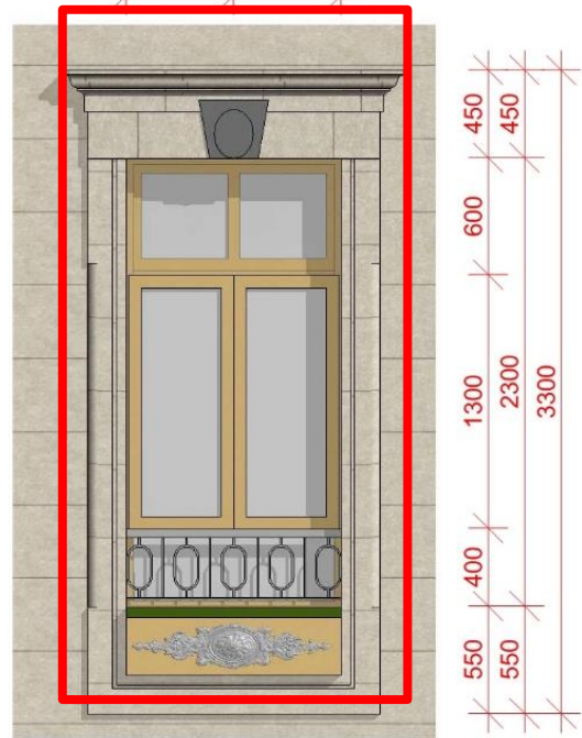
WINDOW ELEVATION B
