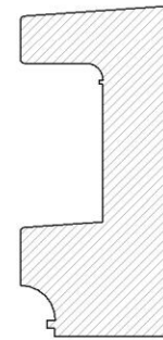
3 PORTICO WINDOW PROFILE 1 : 10
