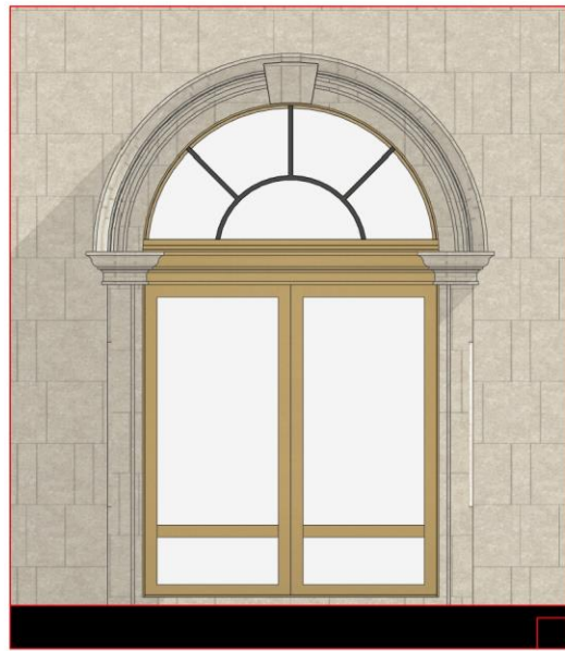
5 SIDE PORTICO WINDOW ELEVATION
